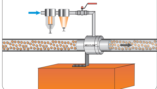
A Model 30004S Stainless Steel 2" Ring Vac™ Air operated conveyor moves dried peas at a pet food manufacturing facility.
